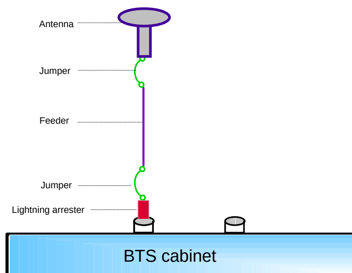
Figure 4-2 Structure of satellite synchronization antenna & feeder
