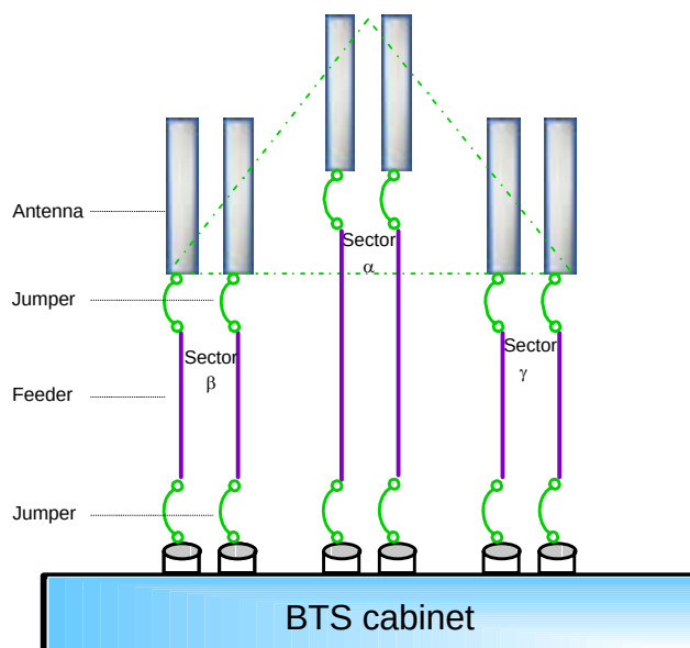
Figure 4-1 Structure of RF antenna & feeder
