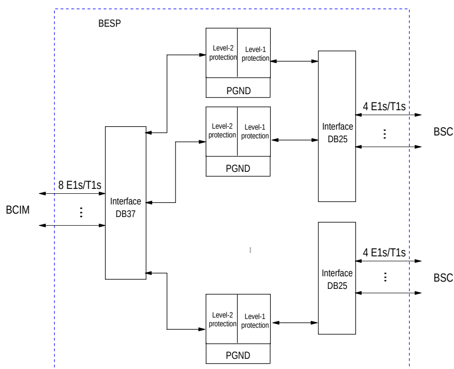
Figure 2-7 Structure of BESP
