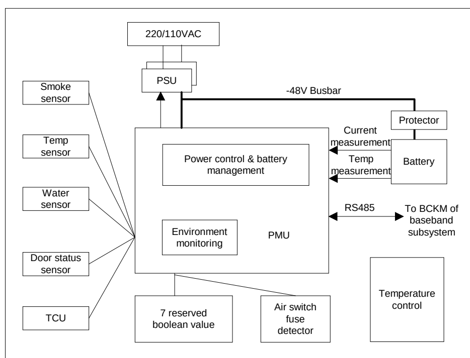
Figure 5-6 Monitoring system of BTS3612A
