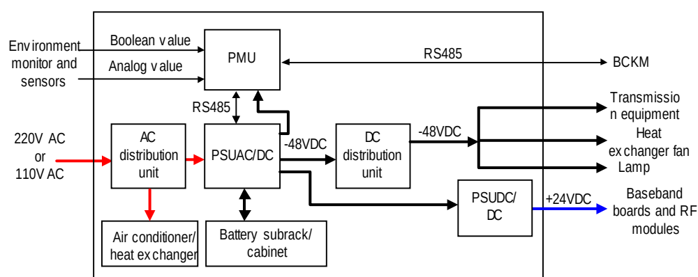
Figure 5-1 Functional structure of the power & environment monitoring subsystem
