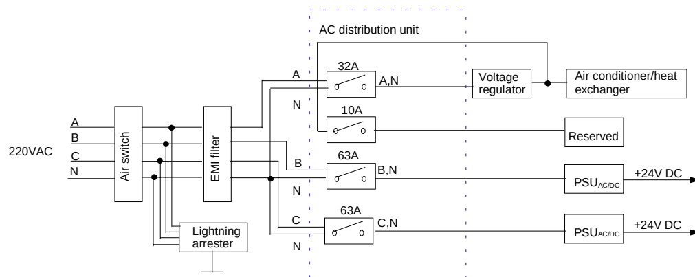
Figure 5-2 Distribution of three-phase 220V AC
