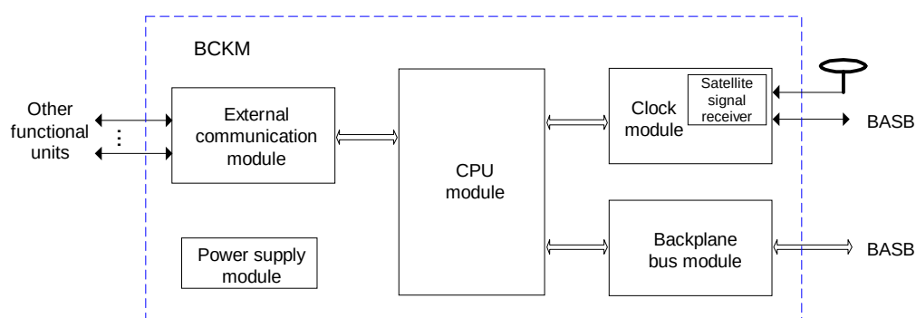
Figure 2-2 Structure of BCKM module
