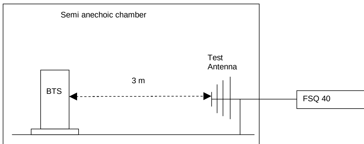
Figure 11. Test set up
