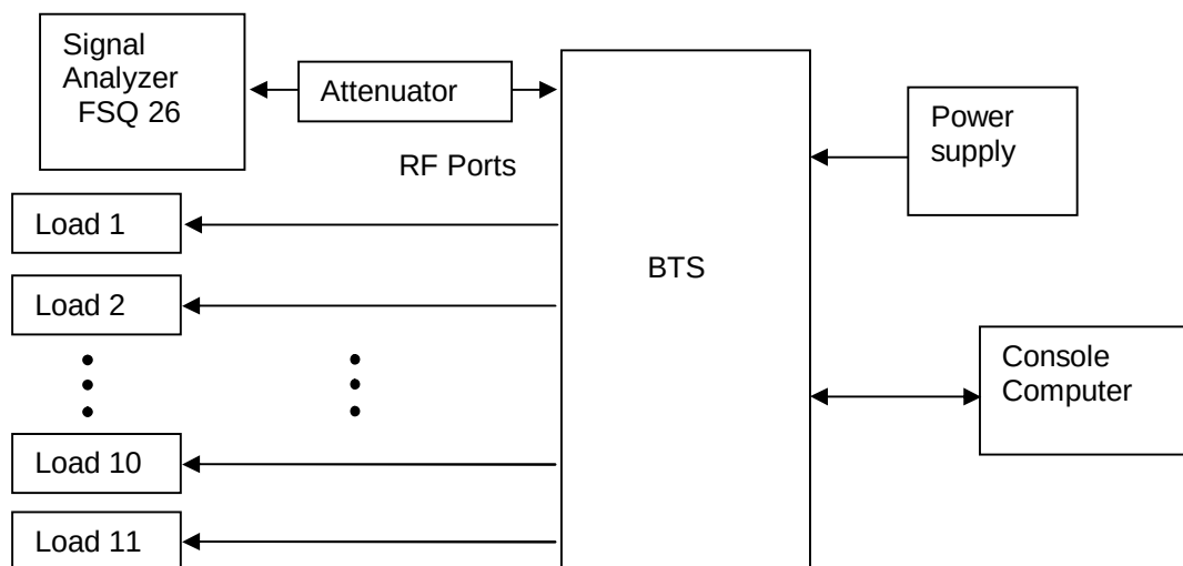
Figure 1. TEST SETUP
