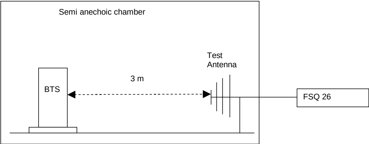
Figure 6. Test setup Step 1
