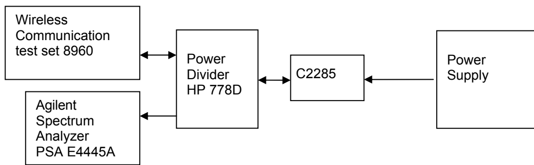
Figure 3. Test Set-up
