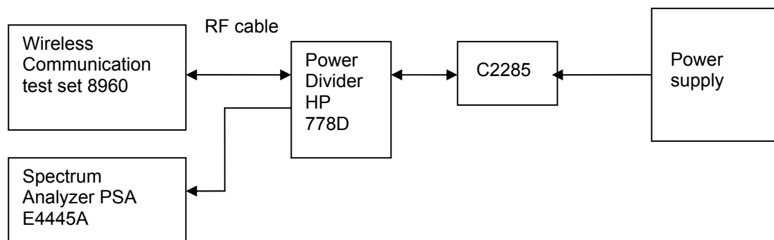
Figure 4. Test Set-up
