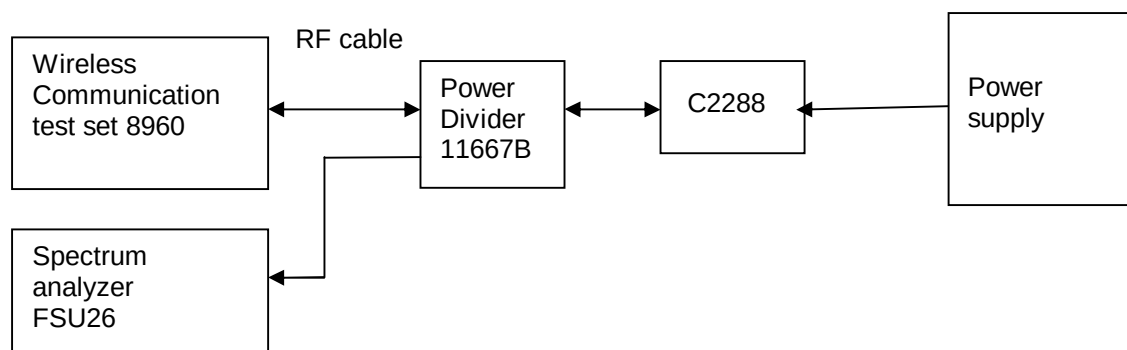
Figure 4. Test Set-up
