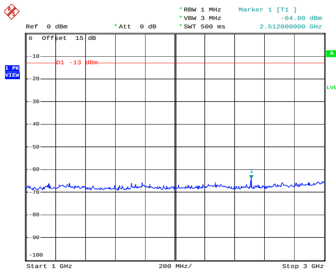
Conducted Emission Plot between 1GHz ~ 3GHz
