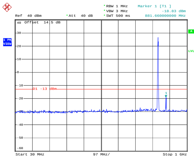
Conducted Emission Plot between 30MHz ~ 1GHz
