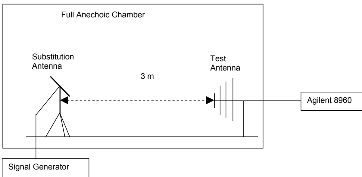
Figure 1. Test Set-up
