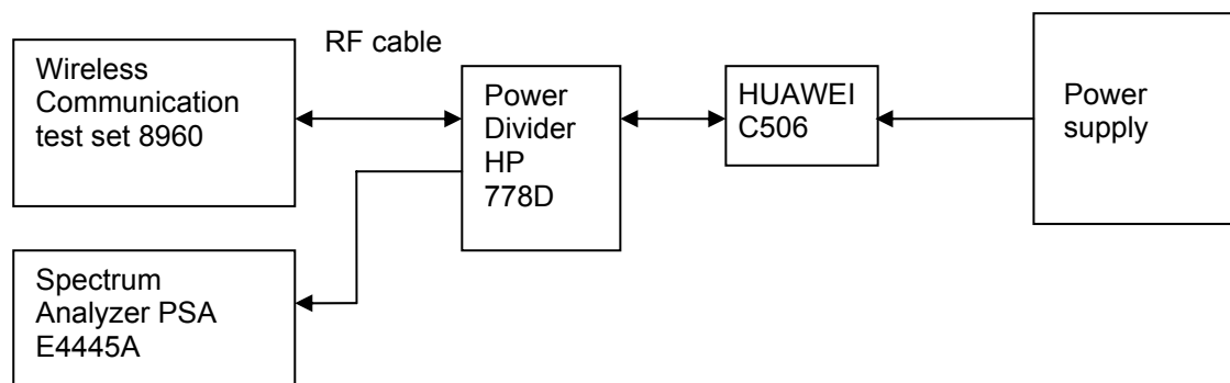
Figure 4. Test Set-up
