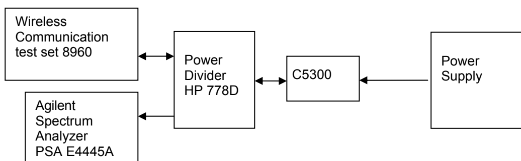
Figure 3. Test Set-up
