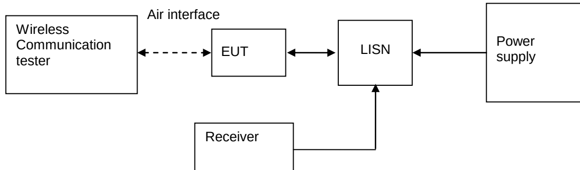
Figure 7. Test Set-up
