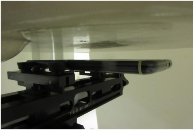
Photo 11: Front Face_15mm
