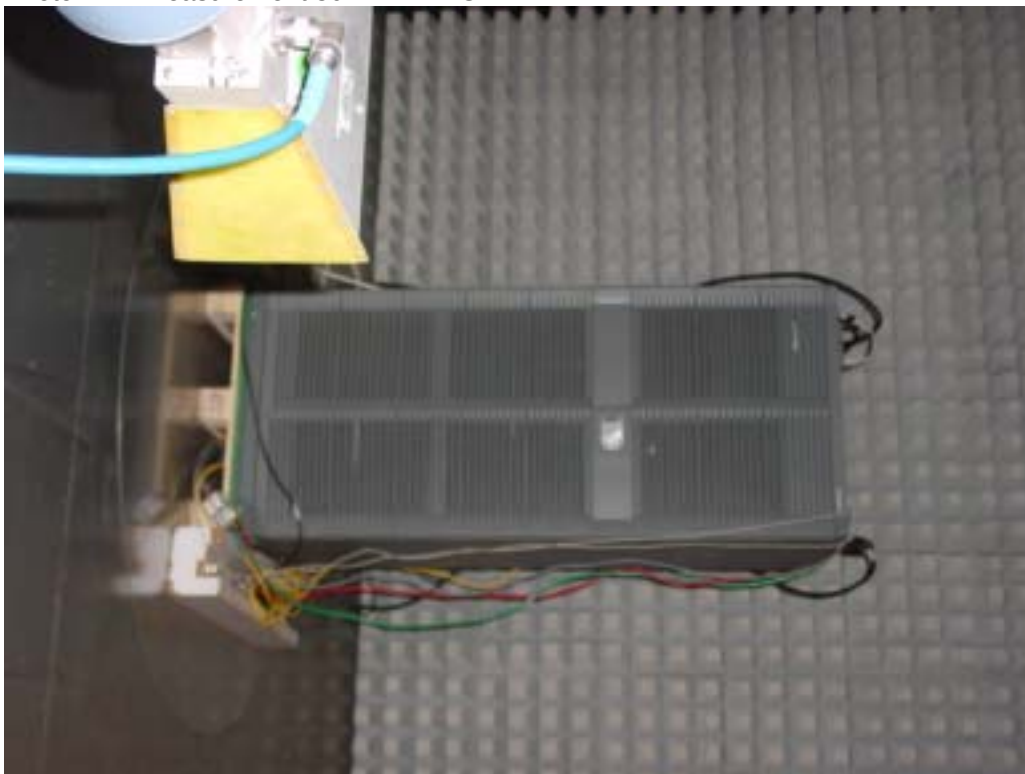
Photo ERP measurement 1 GHz – 10 GHz
