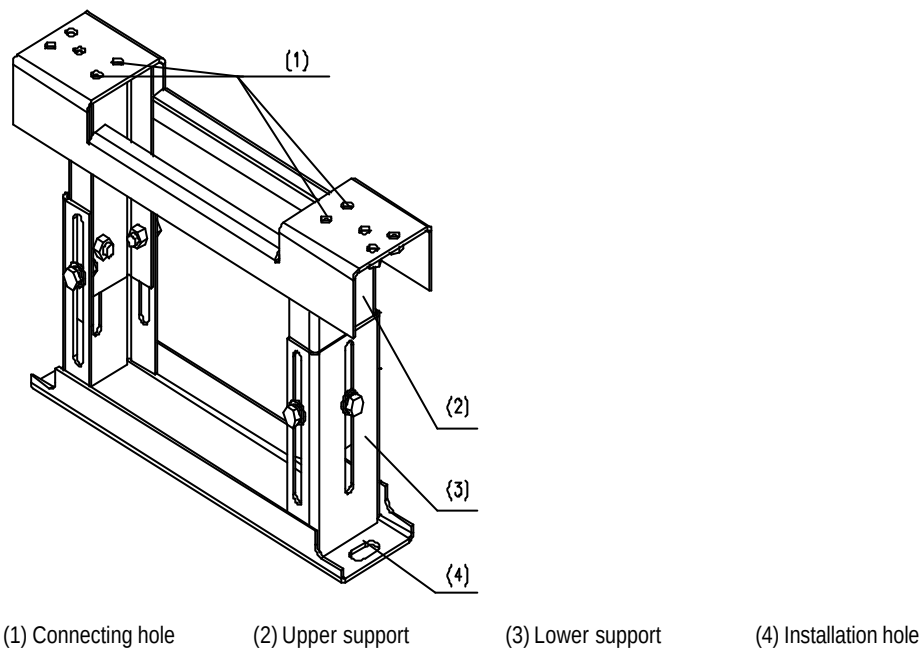
Figure 3-8 Profile of A600 series supports
