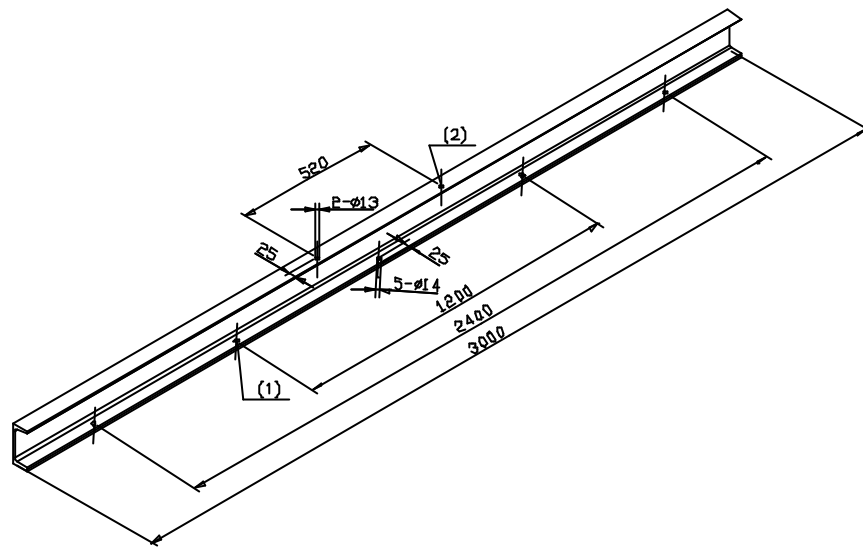
Figure 3-17 Hole fabricating process for U-bar support
