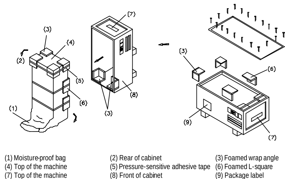
Figure 2-1 Wooden case packing
