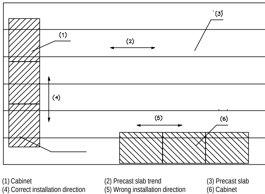
Figure 3-15 Installation direction of combined cabinet
