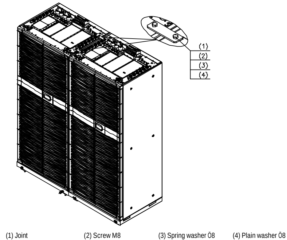
Figure 3-22 Connection of the tops of the combined cabinet
