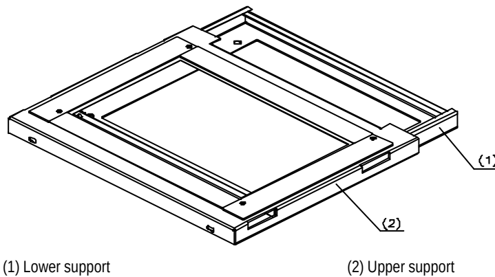
Figure 3-2 Base assembly
