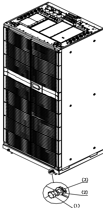
Figure 3-7 cBTS3612 Cabinet installation on the cement floor
