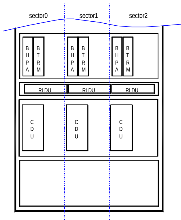
Figure 5-15 S(1/1/1) RF configuration
