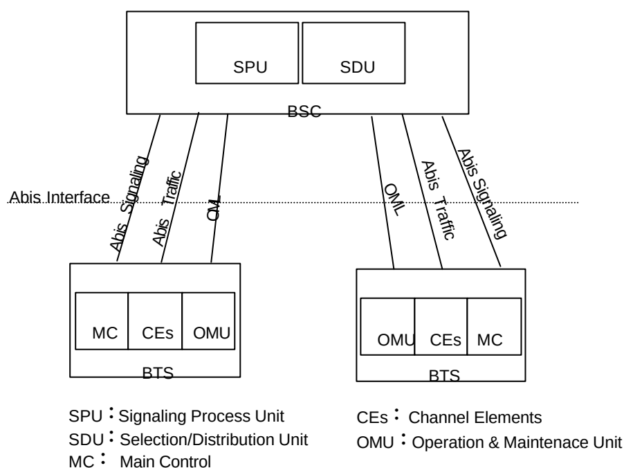
Figure 1-5 Composition of Abis interface
