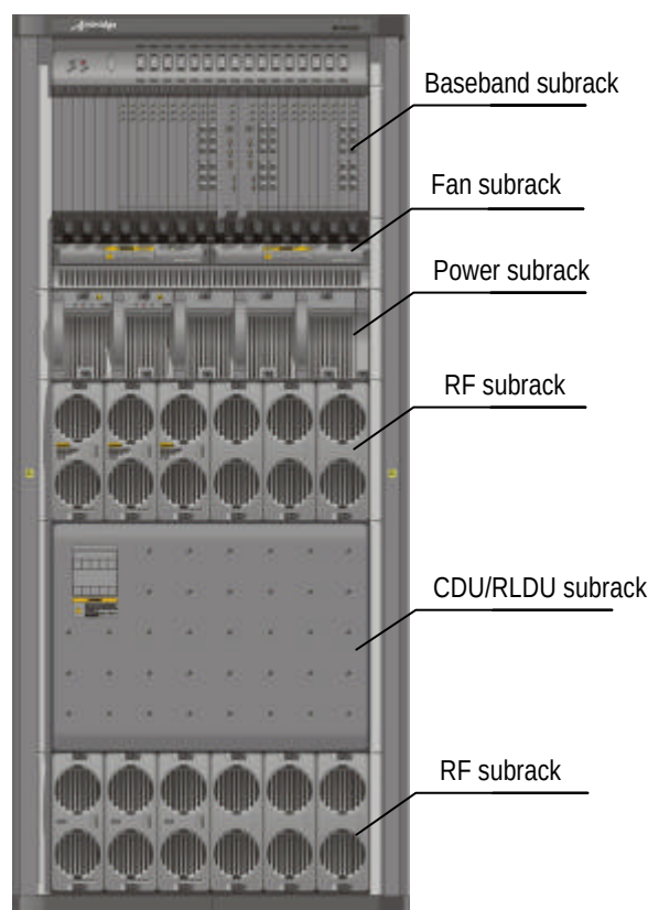
Figure 1-2 cBTS3612 cabinet
