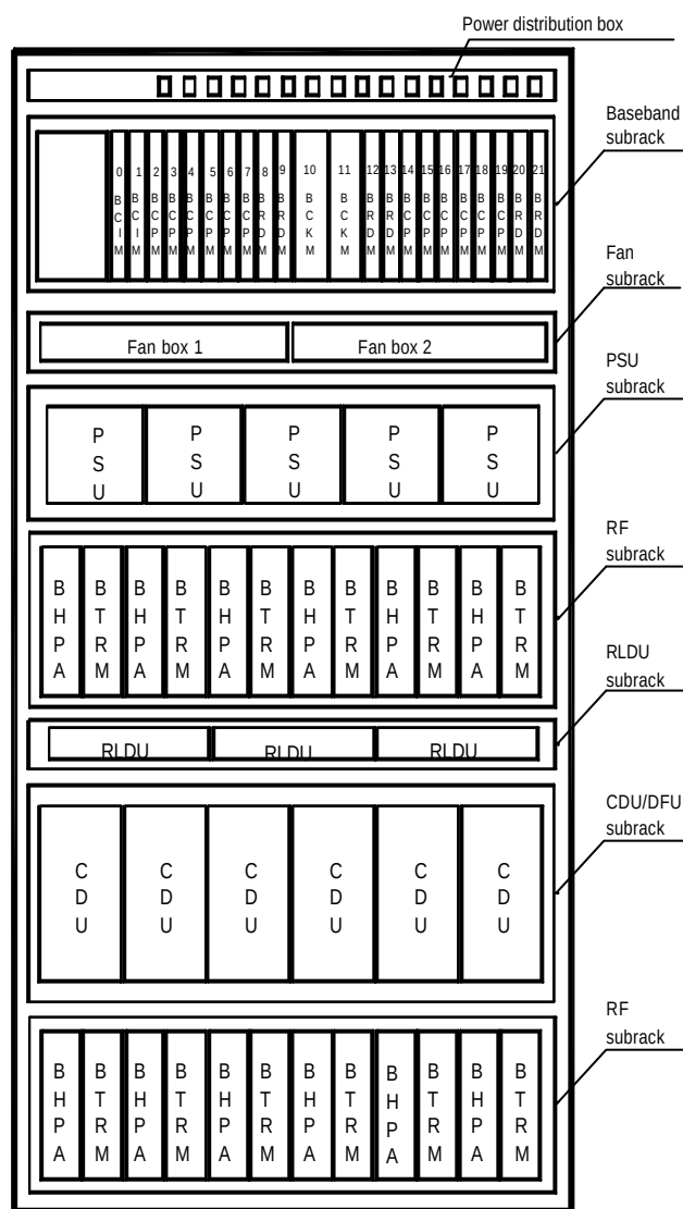
Figure 5-1 Configuration of a basic cabinet
