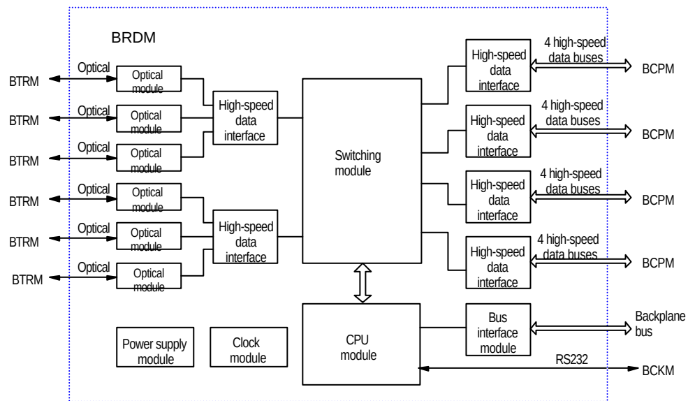
Figure 2-7 Structure of BRDM module
