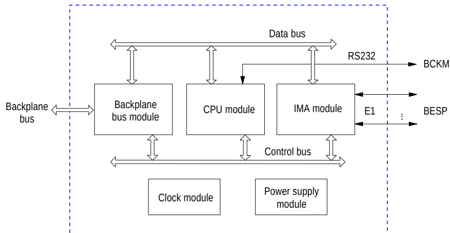
Figure 2-5 Structure of BCIM module
