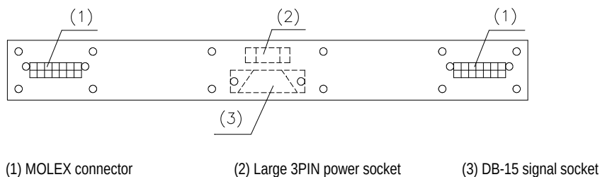
Figure 2-12 Illustration of BFNB structure
