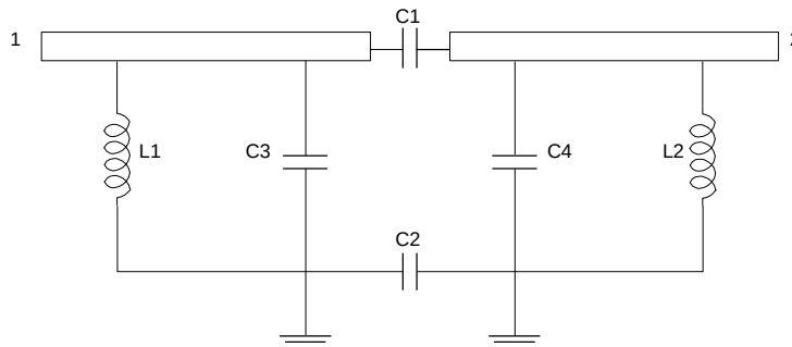
Figure 2-34 Lightning protection for BTS antenna & feeder port
