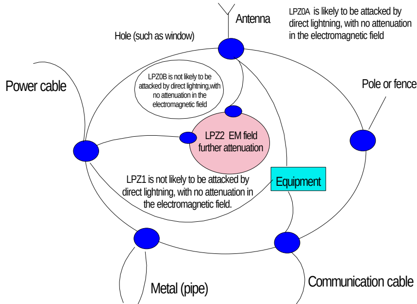
Figure 2-28 IEC 61312 Space division of lightning protection zone
