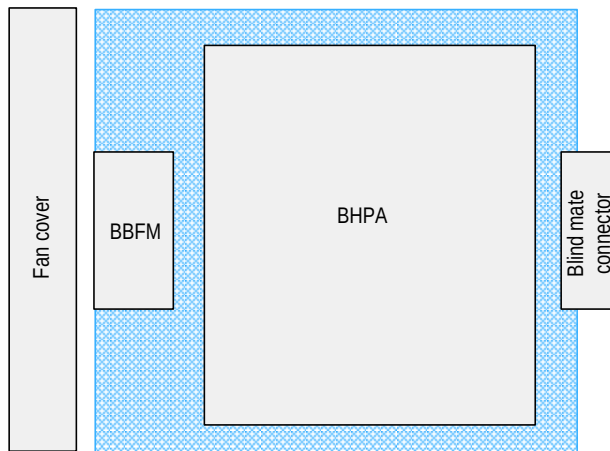
Figure 2-22 Position of BBFM in BHPA module
