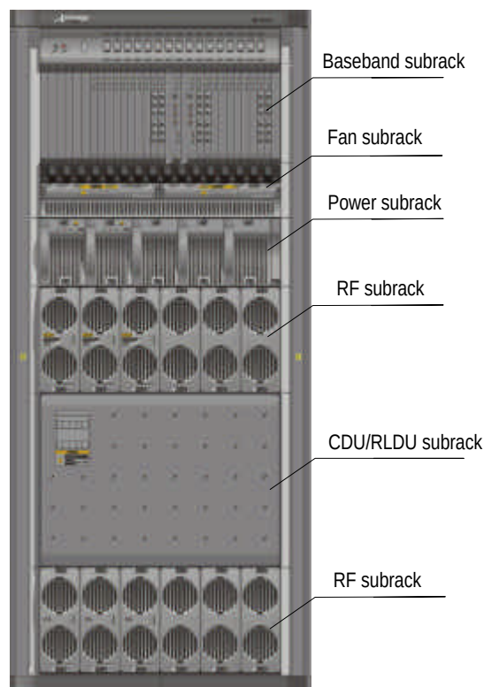
Figure 1-2 cBTS3612-800 cabinet
