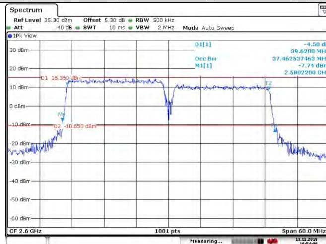
CA_41C_QPSK_100RB+100RB_40591+40789_PCC:100RB@0_SCC:100RB@0
