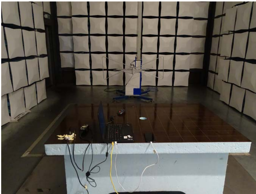
Radiated Disturbance Emissions (below 1GHz)
