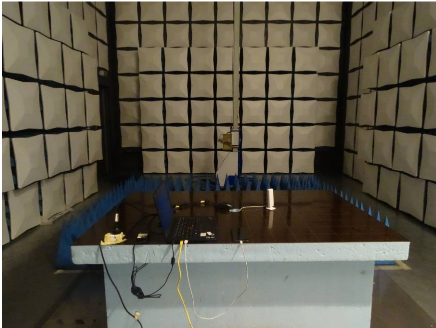
Radiated Disturbance Emissions (1GHz to18GHz)
