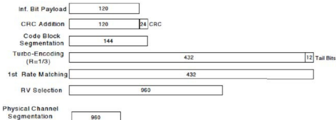
Figure C.8.10: Coding rate for Fixed reference Channel H-Set 12 (QPSK)
