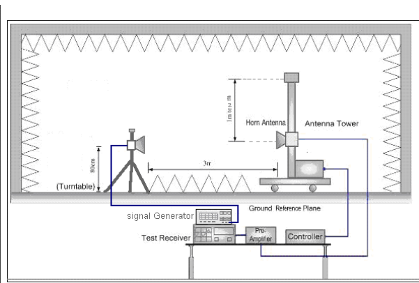
Figure 3. above 1GHz
