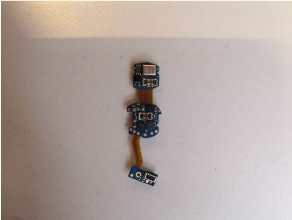
(3) EUT Photo(Earphone-CM-H2)
