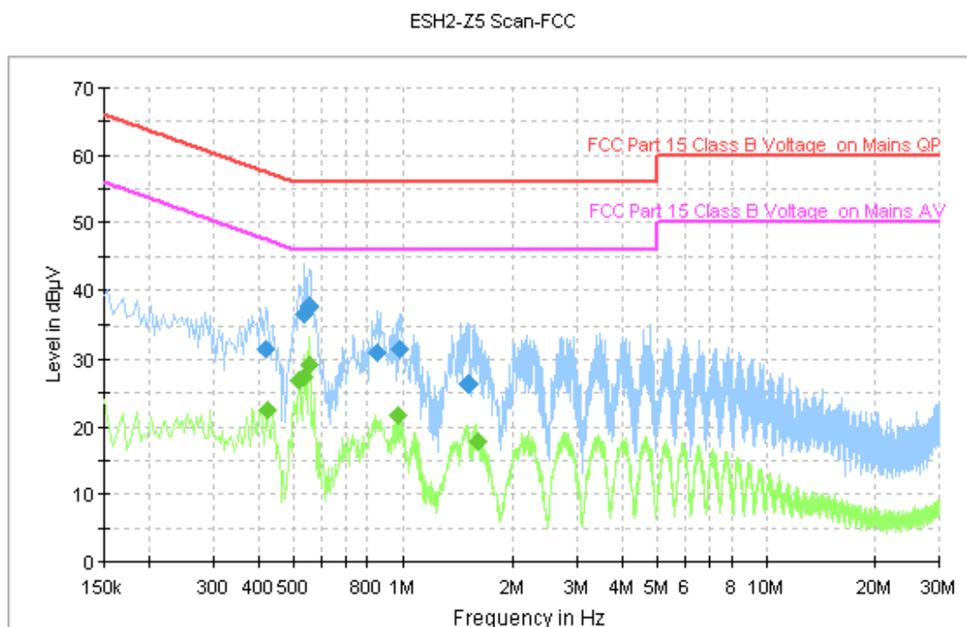
Fig.34 AC Power line Conducted Emission (Idle, AE2)
