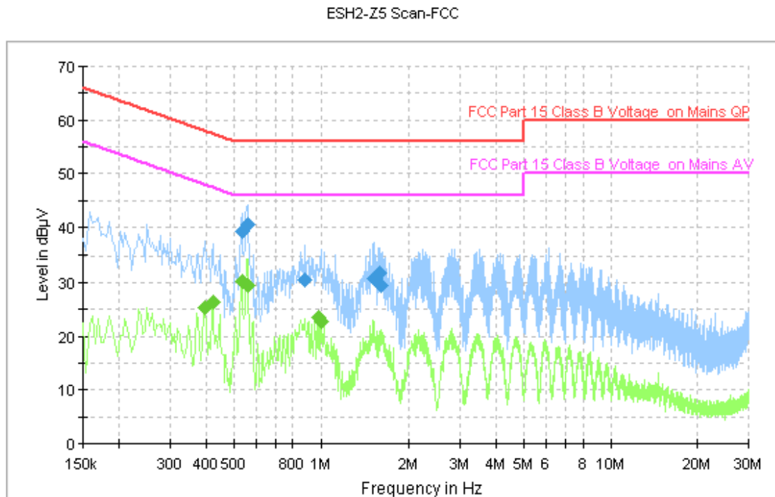
Fig.33 AC Powerline Conducted Emission (Traffic, AE2)
