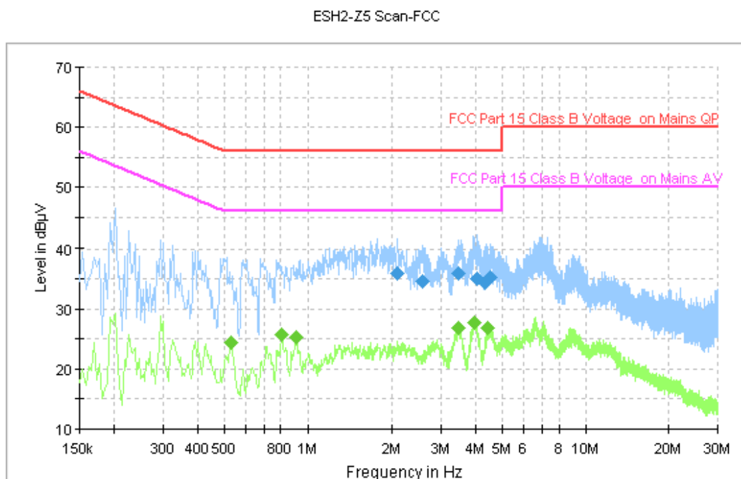
Fig.35 AC Powerline Conducted Emission (Traffic, AE3)
