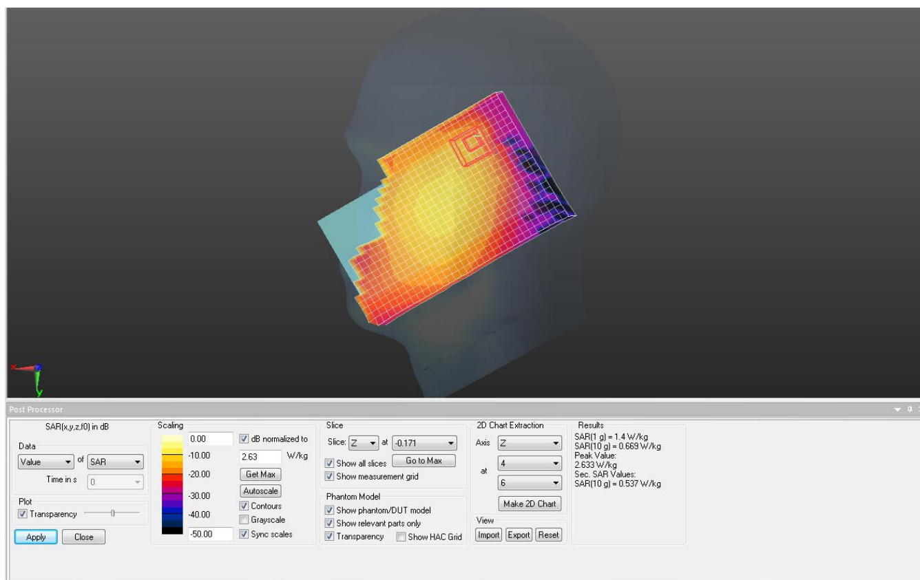
Figure : The volume scan simultaneous transmission SAR test result
