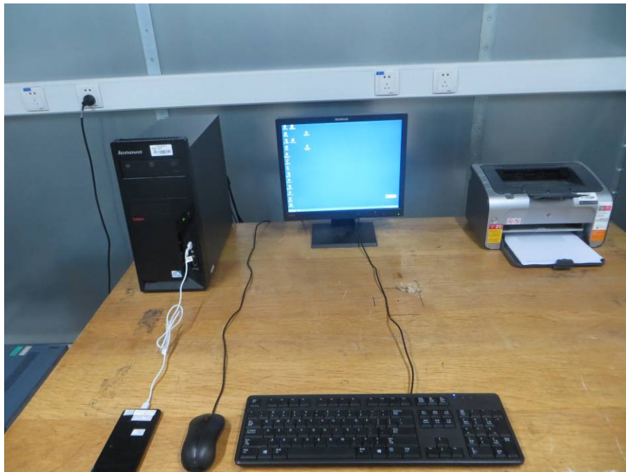
5. Conducted Emission (Part 15B PC mode)
