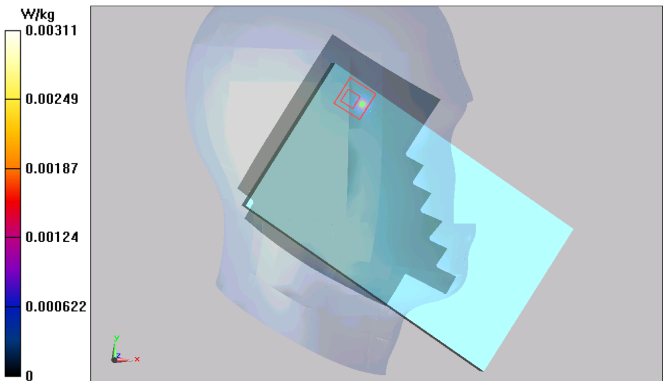
Figure 52 Left Hand Tilt 15^\circ 802.11b Channel 6
