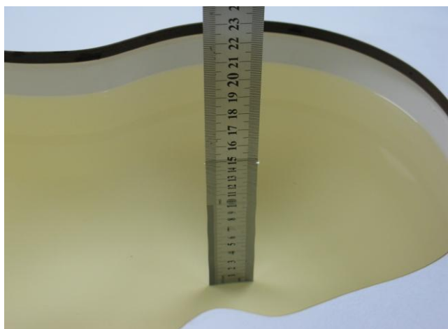
Photo 15:HSL1900MHz depth (15.0cm)
