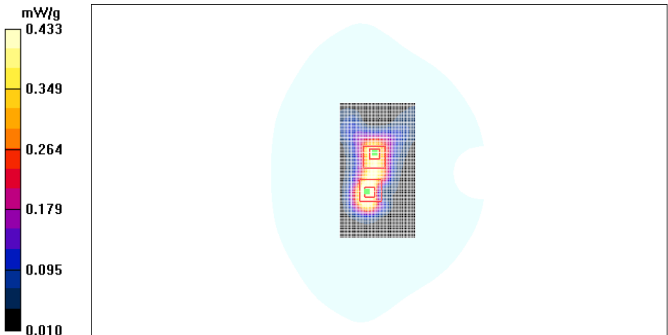
Figure 29 GSM 1900 GPRS (4 timeslots in uplink) with BenQ Joybook S72 Test Position 1 Channel 661
