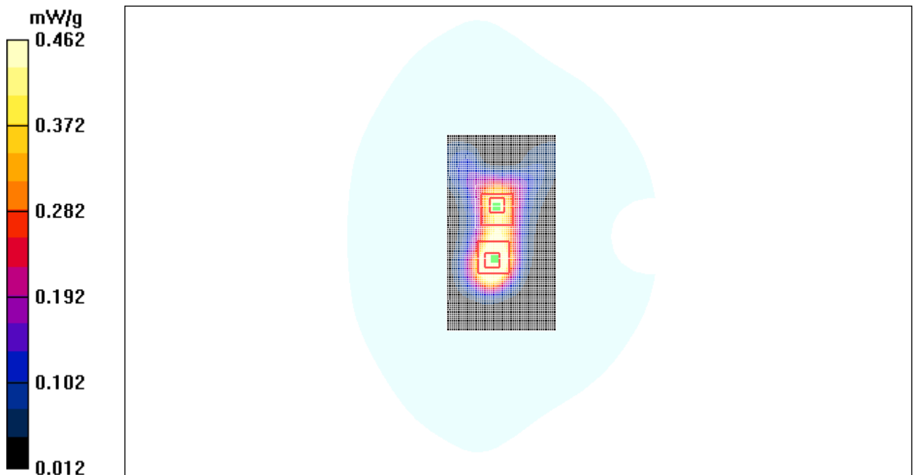
Figure 35 GSM 1900 GPRS (1 timeslot in uplink) with BenQ Joybook S72 Test Position 1Channel 661
