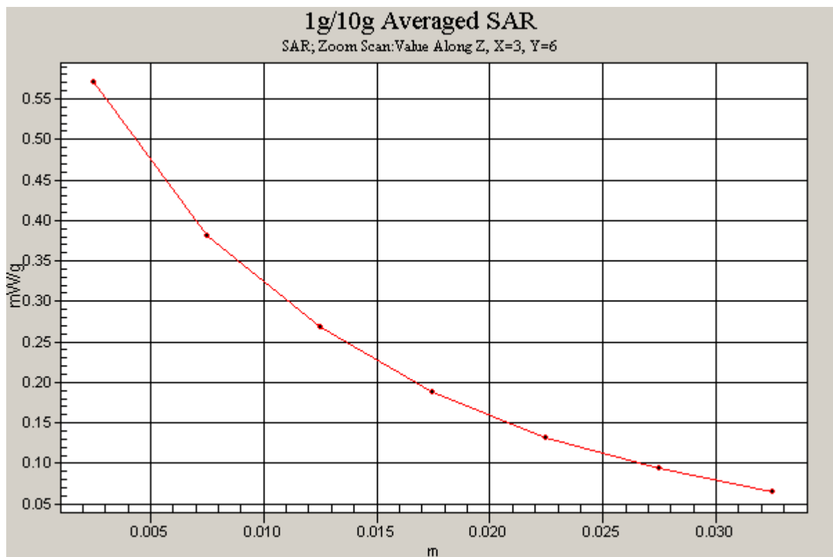
Figure 8 Z-Scan at power reference point [GSM 850 GPRS (4 timeslots in uplink) with BenQ Joybook R55V Test Position 1Channel 192]
