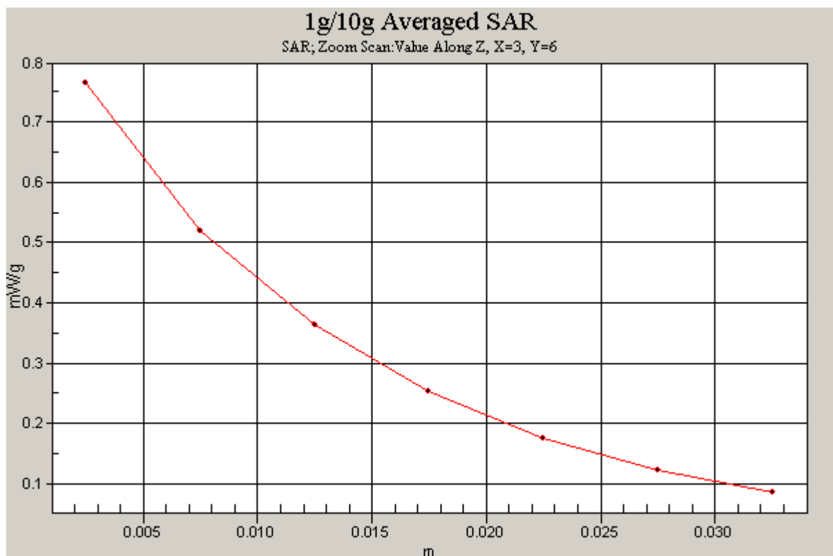
Figure 18 Z-Scan at power reference point [GSM 850 GPRS (1 timeslot in uplink) with BenQ Joybook R55V Test Position 1Channel 192]
