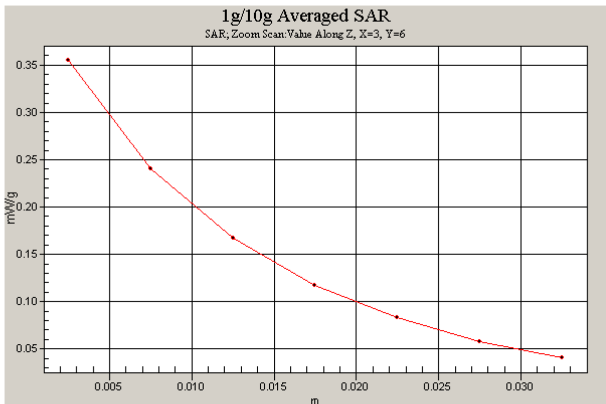
Figure 28 Z-Scan at power reference point (GSM 850 EGPRS (2 timeslots in uplink) with BenQ Joybook R55V Test Position 1 Channel 192
