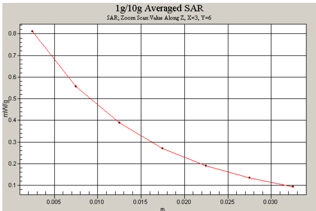
Figure 16 Z-Scan at power reference point [GSM 850 GPRS (2 timeslots in uplink) with BenQ Joybook R55V Test Position 1 Channel 128]
