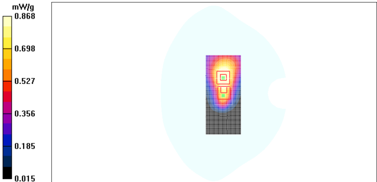
Figure 13 GSM 850 GPRS (2 timeslots in uplink) with BenQ Joybook R55V Test Position 1 Channel 192
