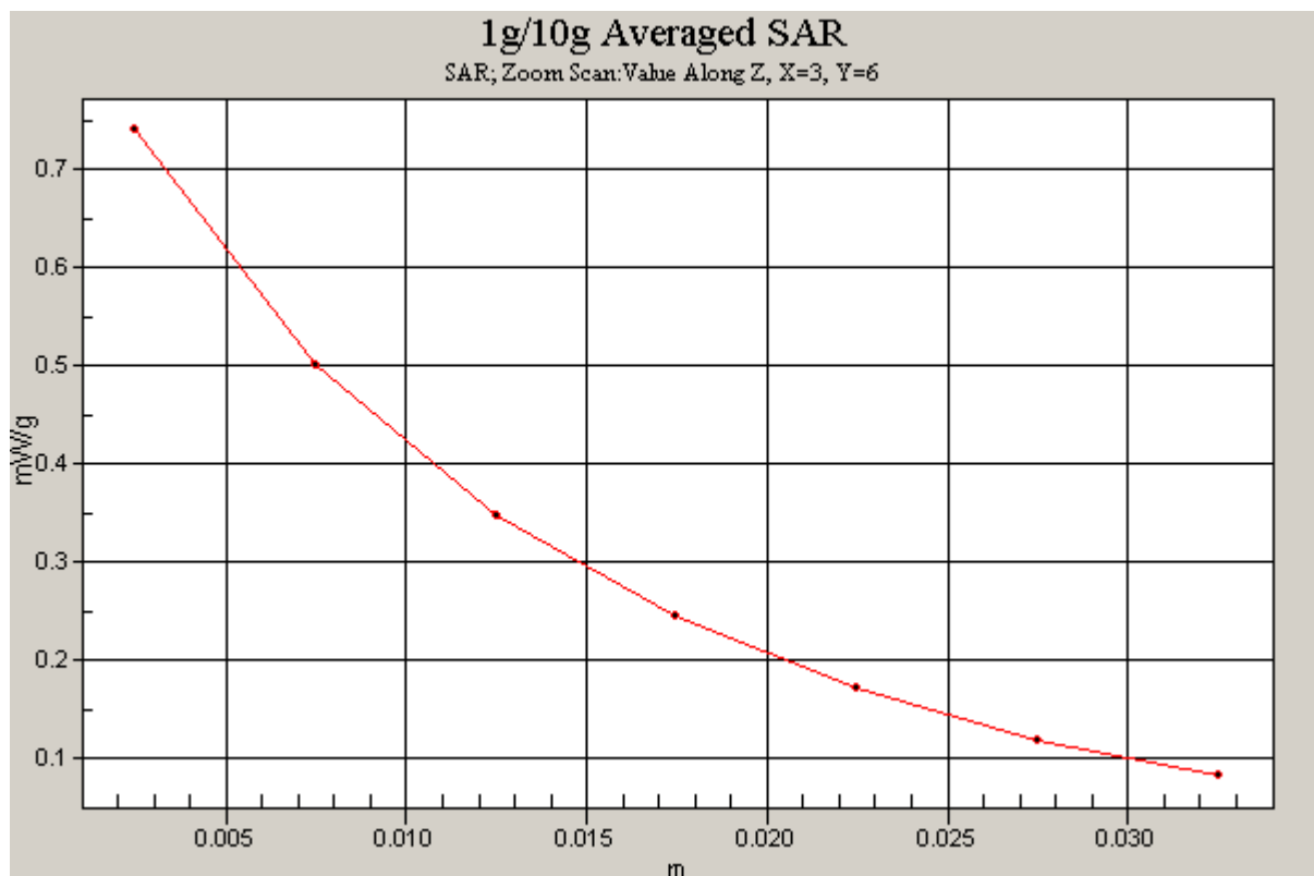
Figure 10 Z-Scan at power reference point [GSM 850 GPRS (3 timeslots in uplink) with BenQ Joybook R55V Test Position 1Channel 192]
