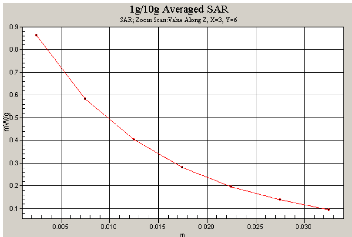
Figure 12 Z-Scan at power reference point [GSM 850 GPRS (2 timeslots in uplink) with BenQ Joybook R55V Test Position 1Channel 251]
