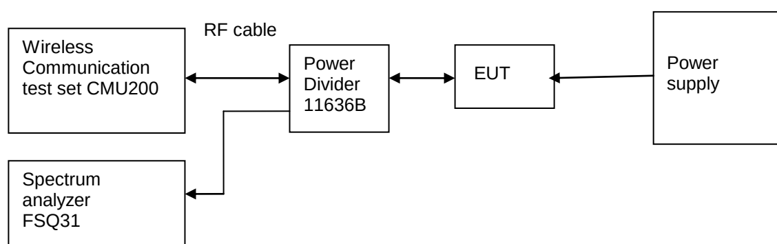
Figure 6. Test Set-up
