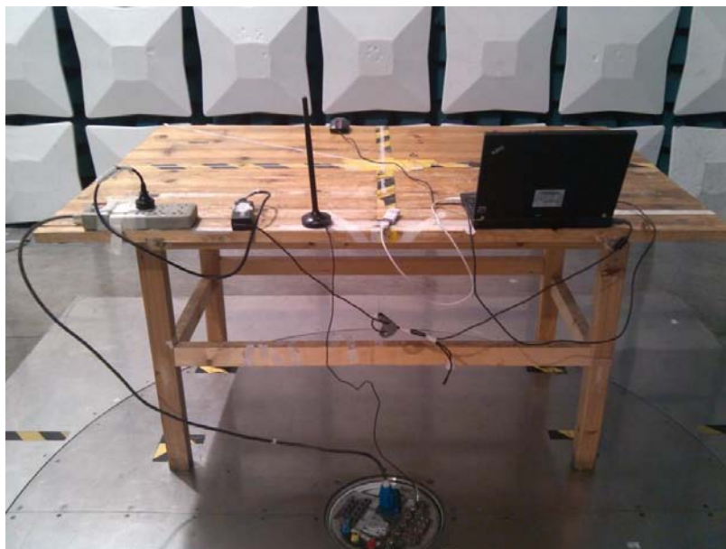
Radiated Disturbance (above 1GHz)
