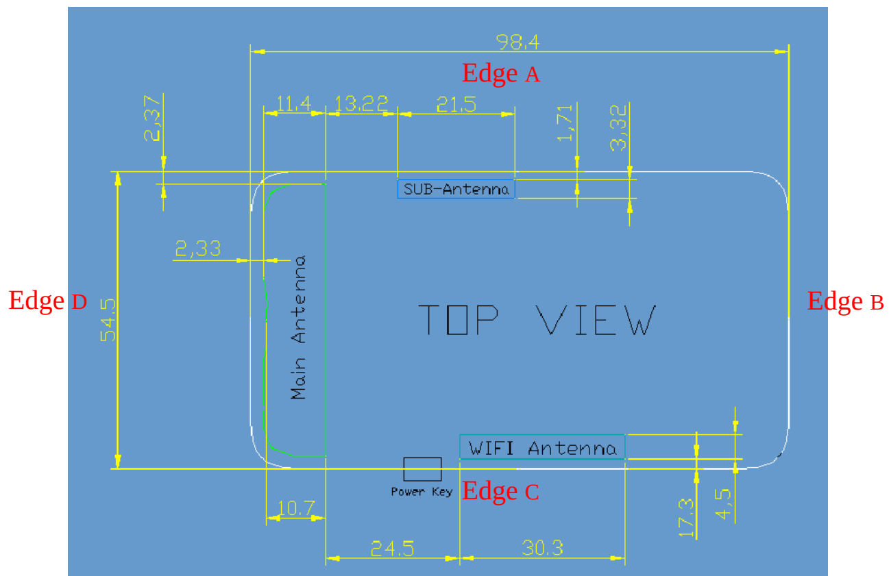
Fig. 3 Position of the antennas
