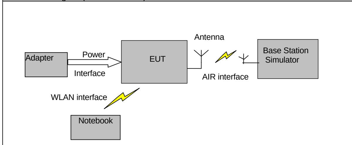
Connection Diagram (Mode 1~Mode 2)
