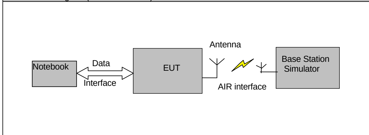
Connection Diagram (Mode 3~Mode 4)
