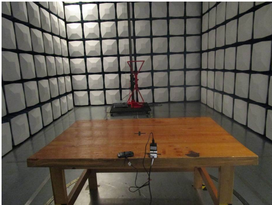
Radiated Emission Below 1GHz Rear View (Charging Mode)
