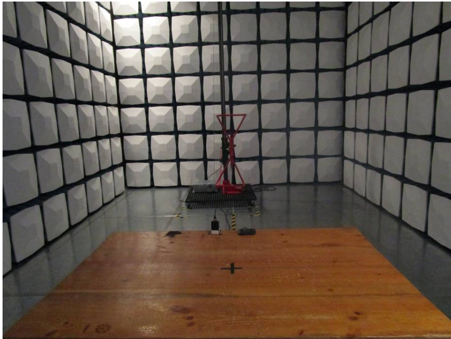
Radiated Emission Below 1GHz Front View (Charging Mode)
