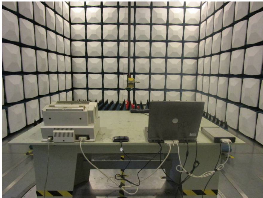
Radiated Emission Above 1GHz Rear View (Downloading Mode)
