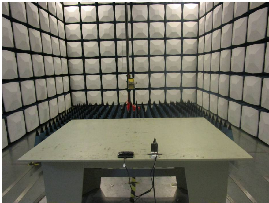
Radiated Emission Above 1GHz Rear View (Charging Mode)
