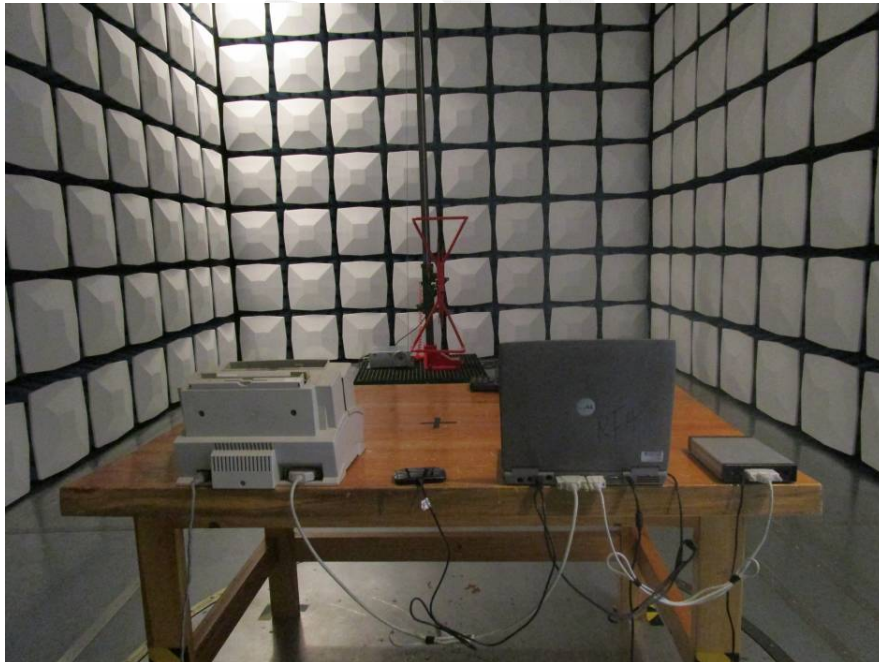
Radiated Emission Below 1GHz Rear View (Downloading Mode)
