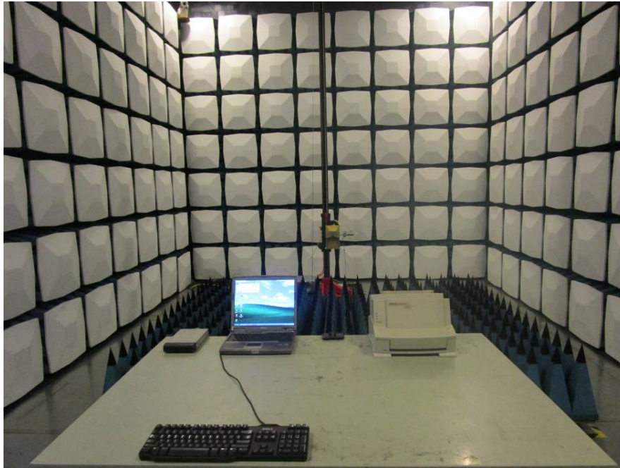
Radiated Emission Above 1GHz Front View (Downloading Mode)
