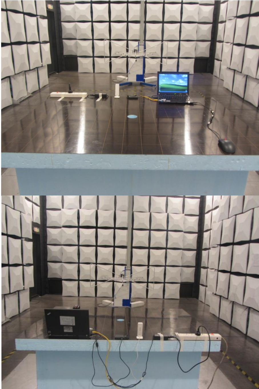
Radiated Disturbance (30MHz To 1GHz)
