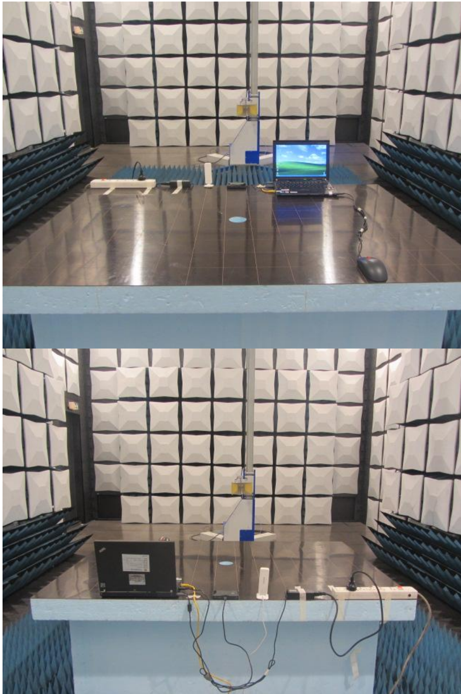
Radiated Disturbance (1GHz To 18GHz)
