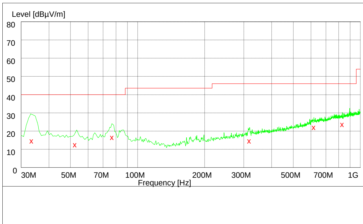
MEASUREMENT RESULT: QP Detector
