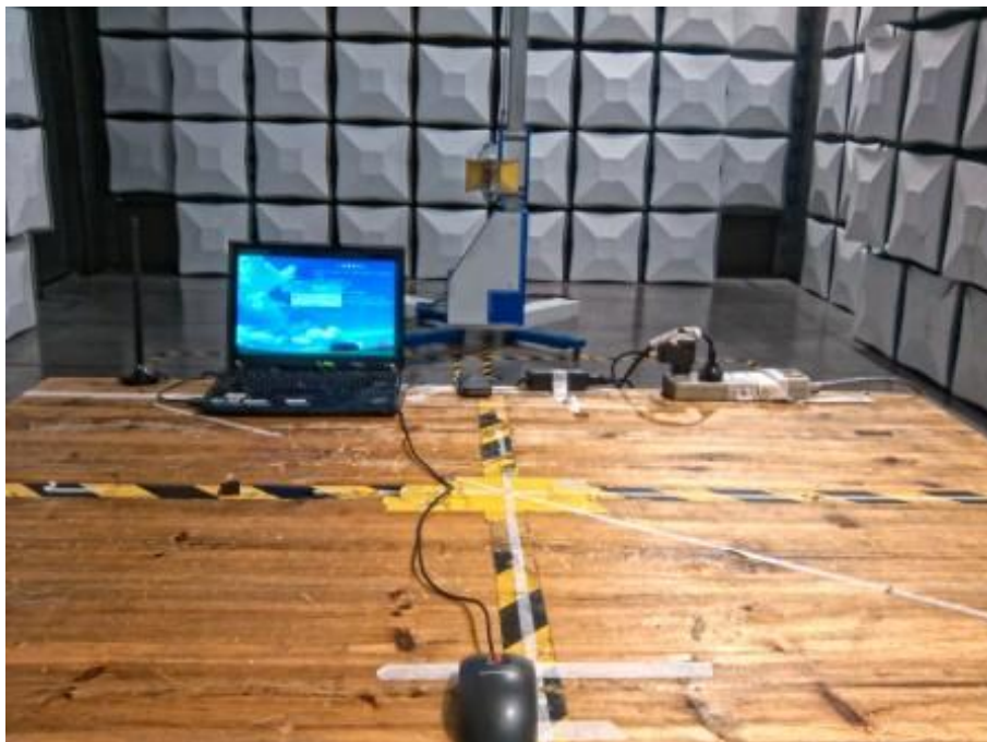
Radiated Disturbance (1GHz-18GHz)
