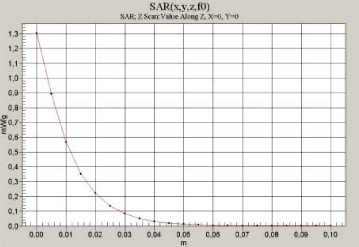
Z-Axis scan 1900 MHz body
