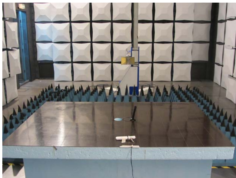
Car Charger Radiated Disturbance Emissions (1GHz to 18GHz)
