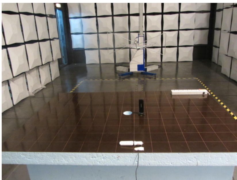
Car Charger Radiated Disturbance Emissions (below 1GHz)
