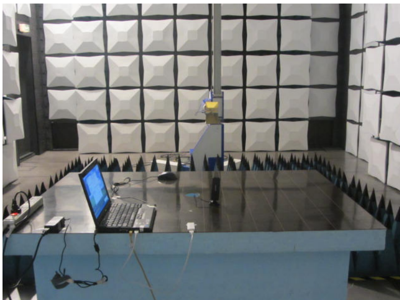
Radiated Disturbance Emissions (1GHz to 18GHz) for PC mode
