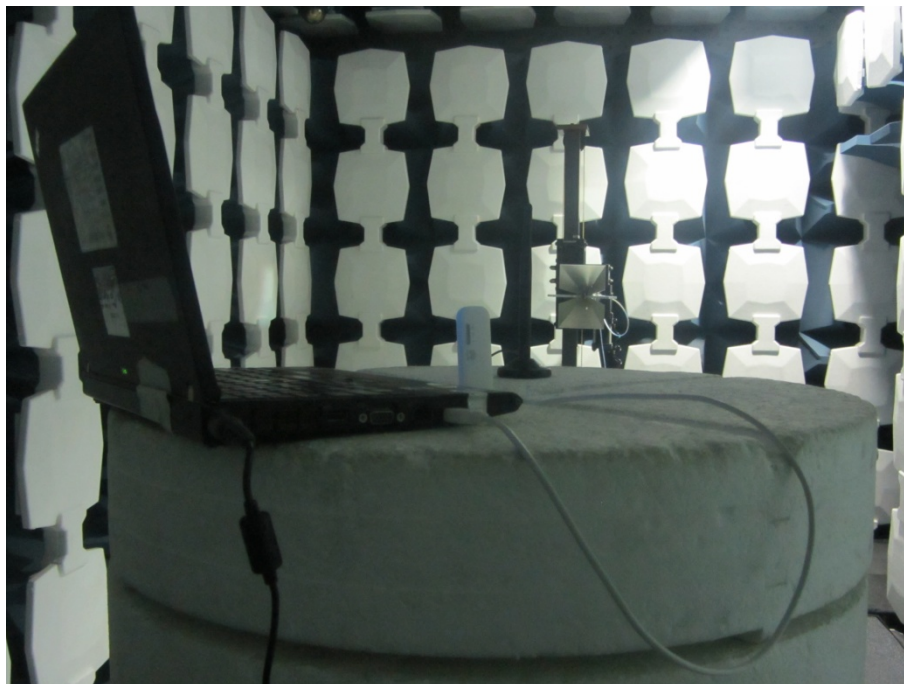
Radiated Spurious Emission (3GHz to 18GHz)
