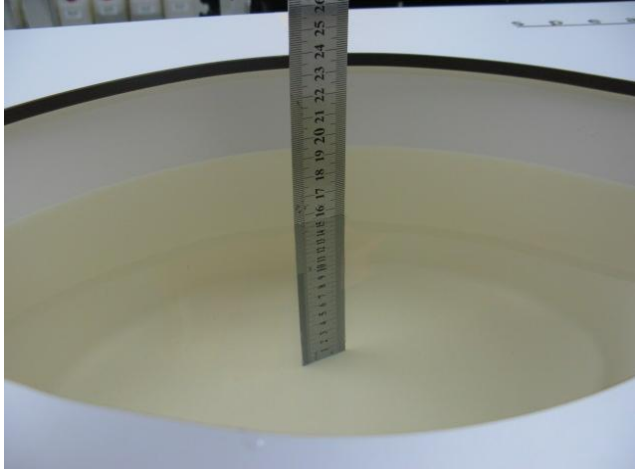
Photo 11: MSL 2450MHz depth (15.3cm)
