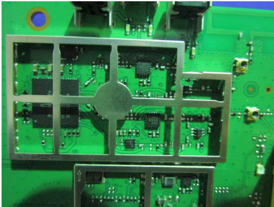
EUT –Wifi RF Chip View
