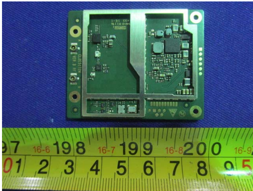
EUT –LTE Module Top Uncover View
