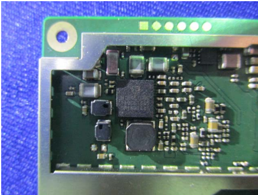
EUT –LTE RF Chip View
