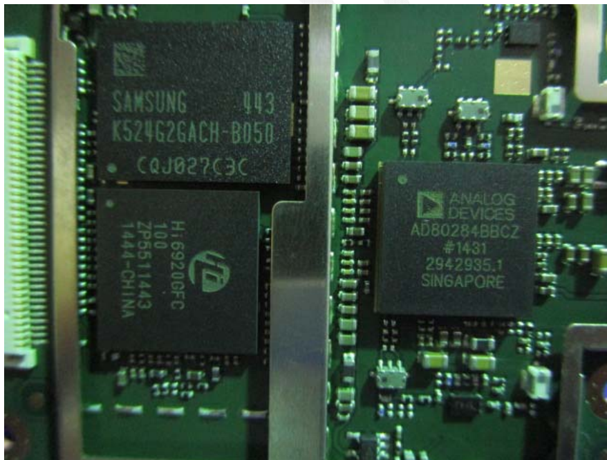
EUT –LTE Main Chip View
