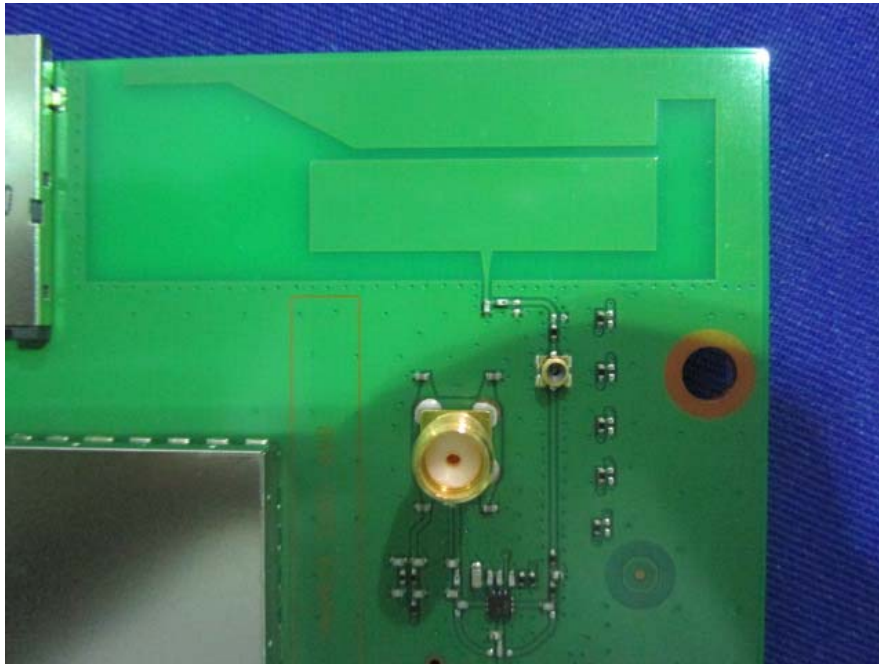
EUT –LTE Internal Antenna View
