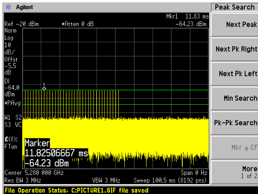
Radar Type 2
