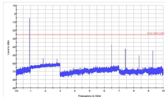
928MHz 30MHz to 10GHz
