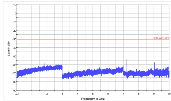
925MHz 30MHz to 10GHz
