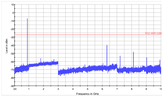
920MHz 30MHz to 10GHz
