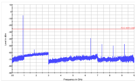
926.7MHz 30MHz to 10GHz
