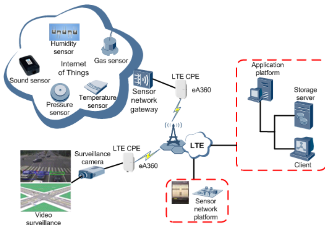
Figure 1-2 The eA360 deployed in industrial private networks
