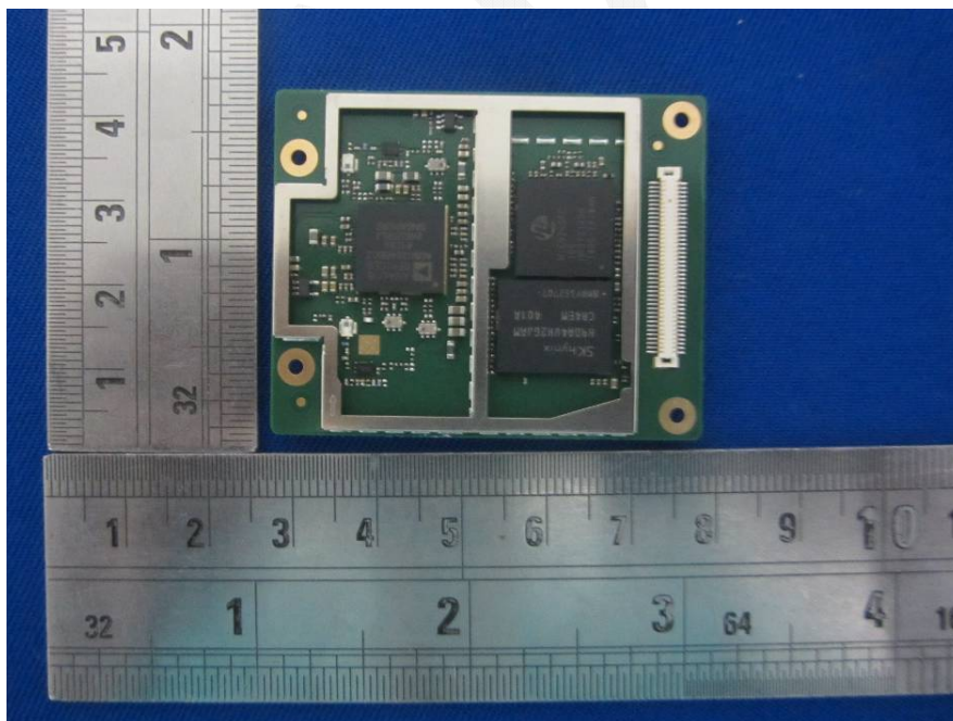
EUT -LTE Module Bottom Without Shielding View
