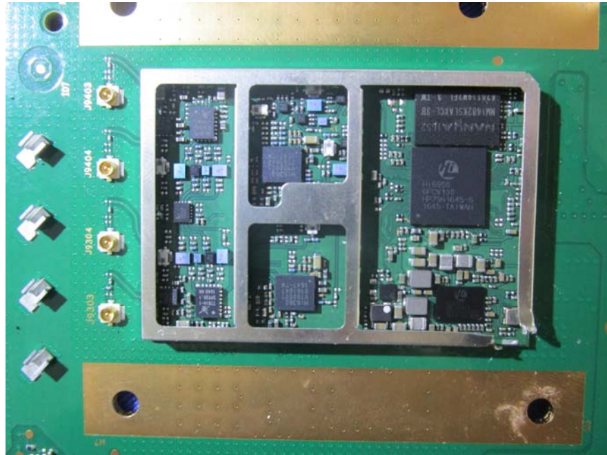
EUT – LTE Module View
