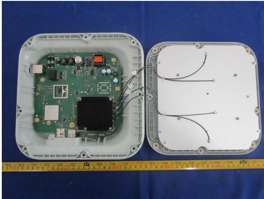
EUT – Case Open 1 View
