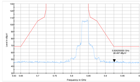
Frequency 5840MHz
