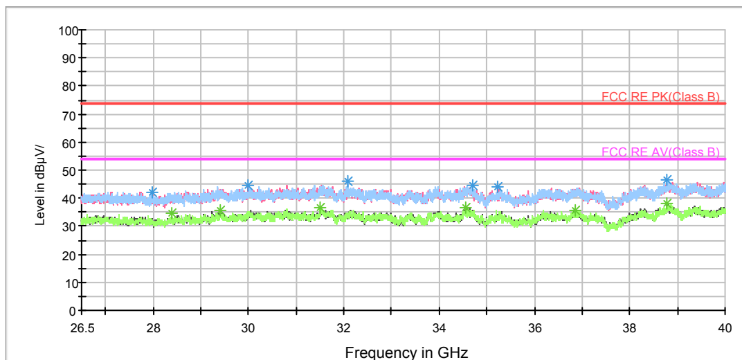
RE 26.5-40GHz PK+AV
