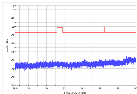
Frequency 5735MHz, 26.5G-40GHz
