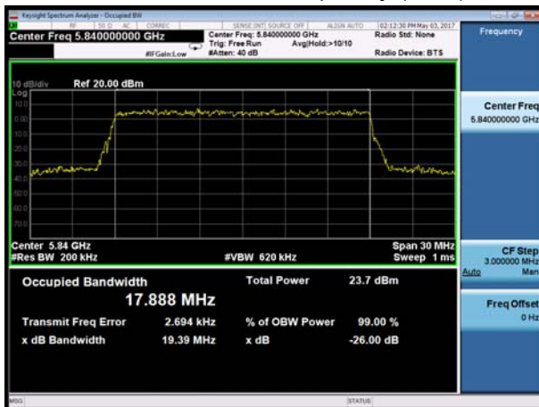
99% bandwidth, Carrier frequency (MHz): 5840
