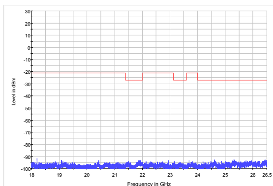
Frequency 5735MHz, 18G-26.5GHz
