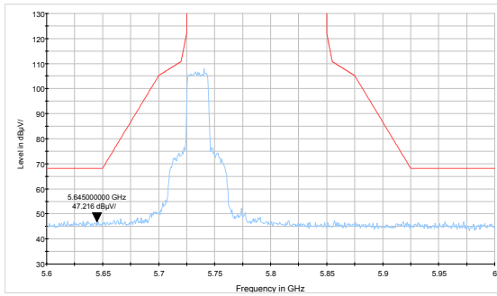
Frequency 5735MHz
