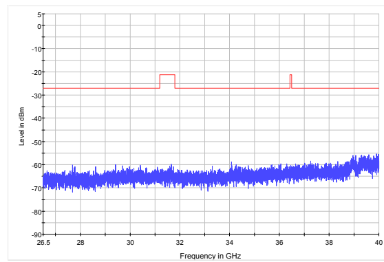
Frequency 5790MHz, 26.5G-40GHz
