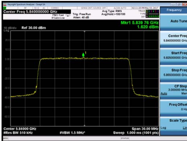
Carrier Frequency (MHz): 5840
