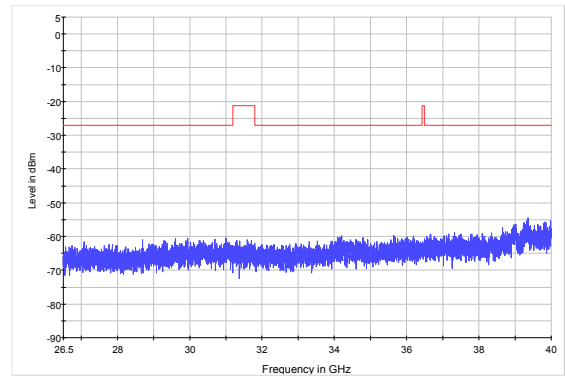
Frequency 5840MHz, 26.5G-40GHz
