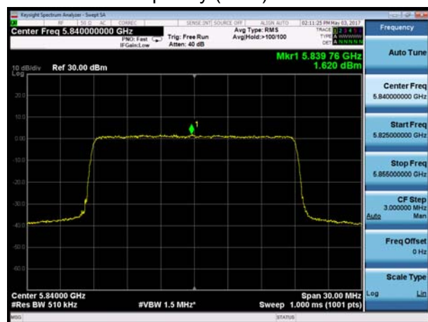
Frequency (MHz): 5840
