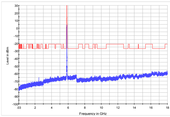
Frequency 5840MHz, 30M-18GHz
