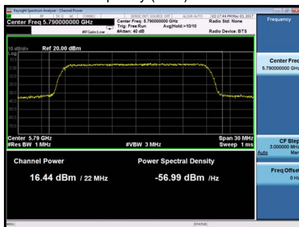
Frequency (MHz): 5790
