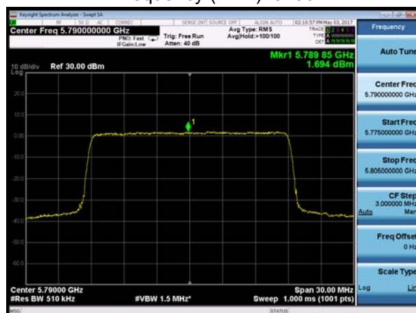
Frequency (MHz): 5790
