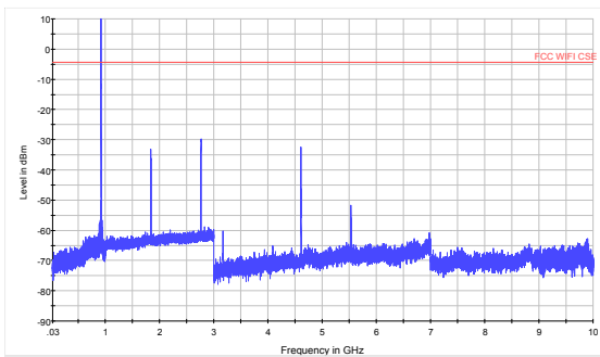
CSE_922MHz_0.03-10GHz
