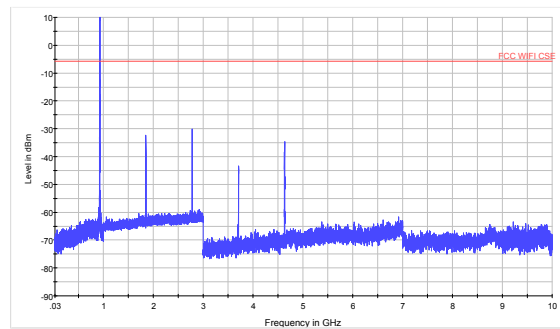
CSE_926.7MHz_0.03-10GHz
