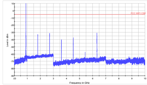
CSE_905MHz_0.03-10GHz
