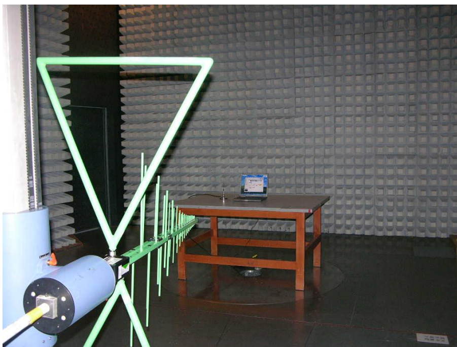
Radiated Disturbance of AC mode (below 1GHz)
