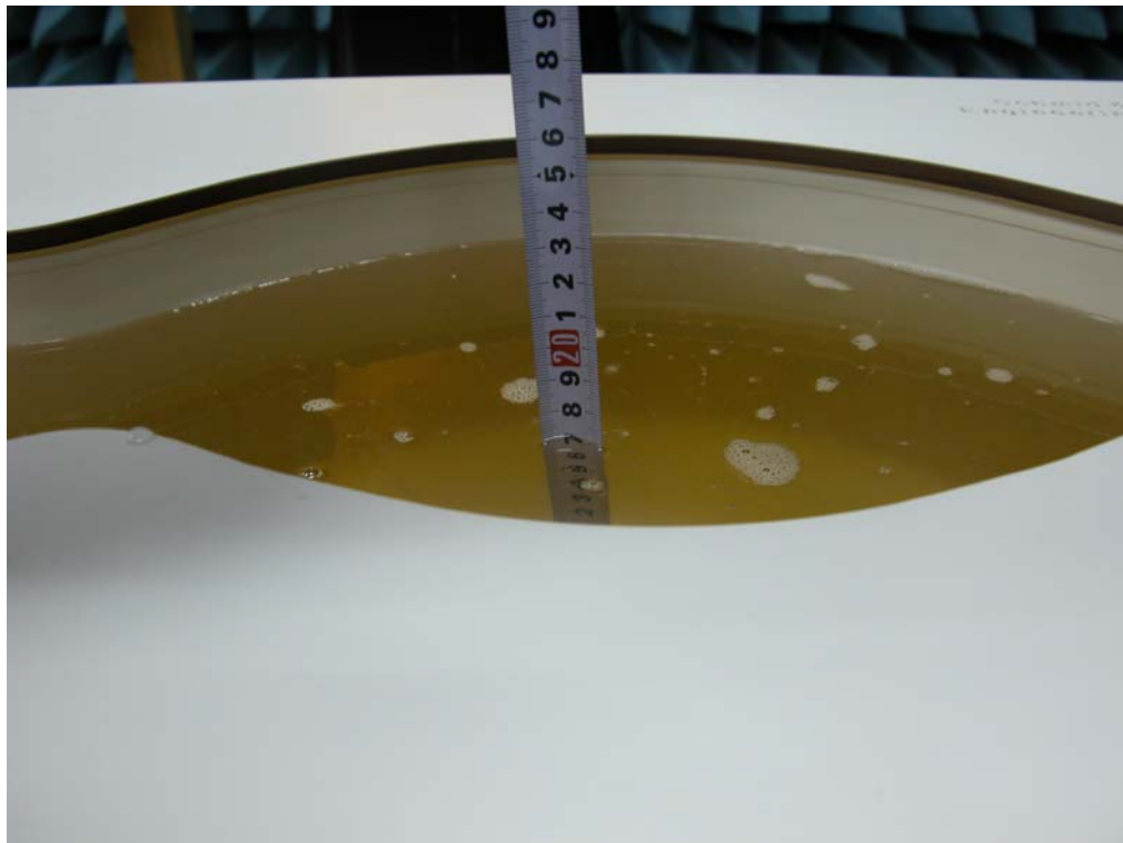
Picture B2: Liquid depth in the Flat Phantom (CDMA 835)
