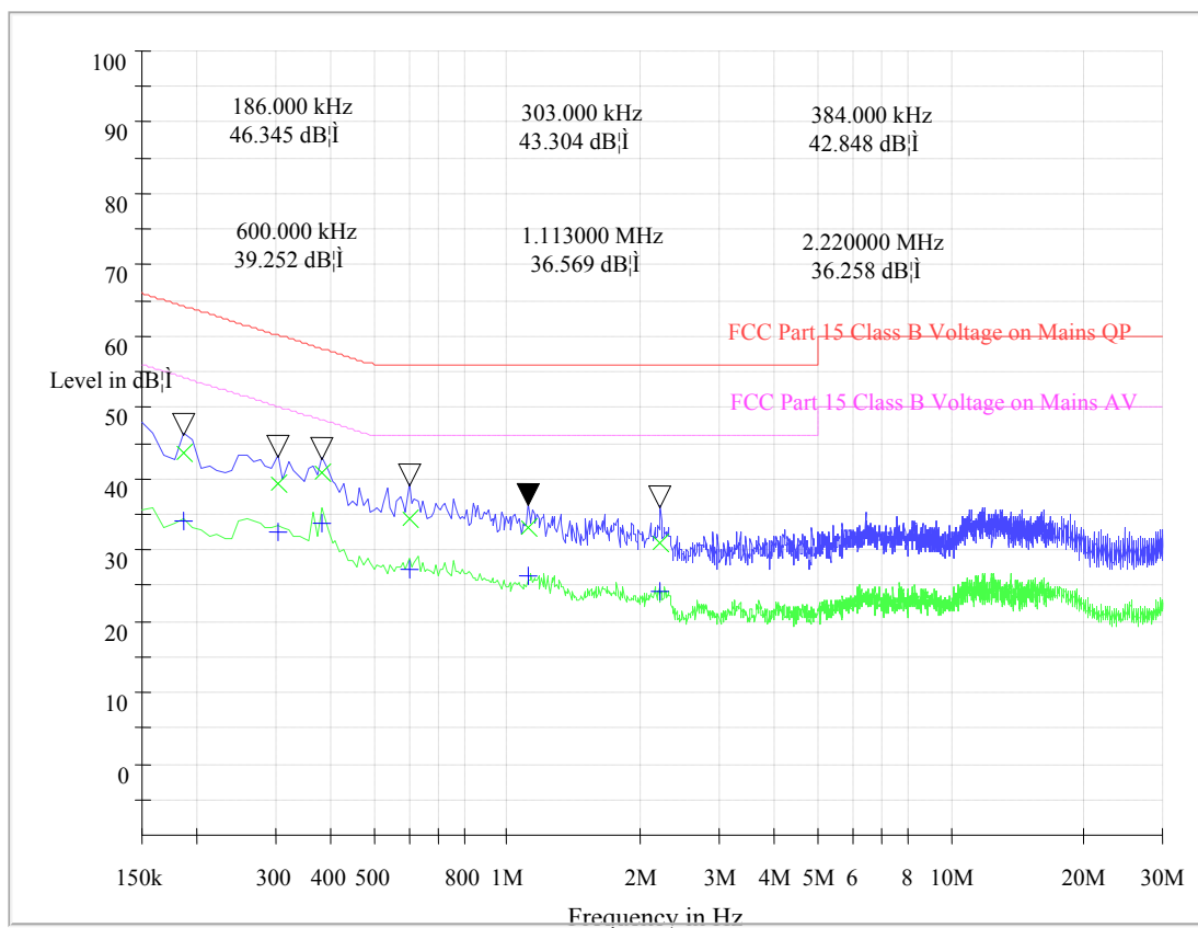
FCC Part 15 Class B Voltage Test
