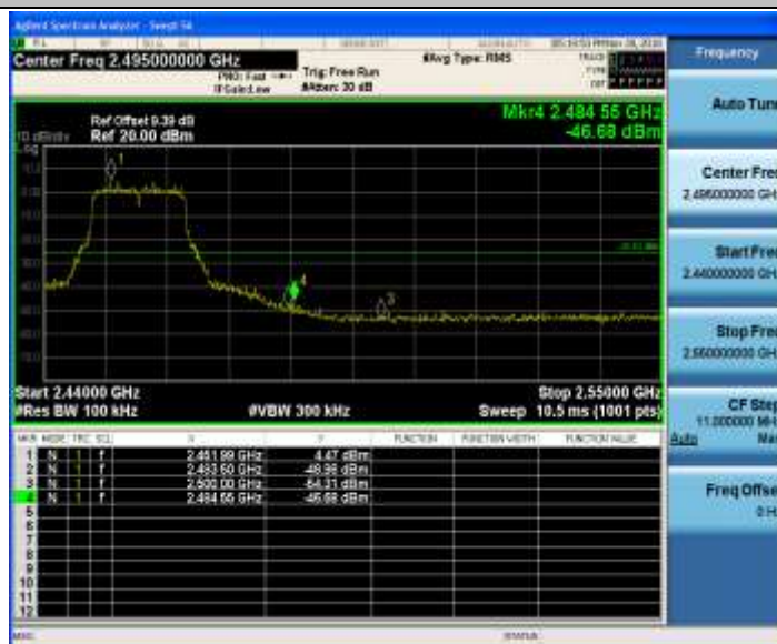
11G-CDD_Ant1_High_2462
